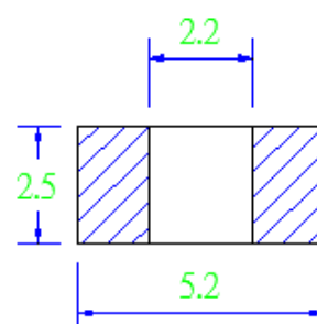
Recommend Land Pattern Dimensions
